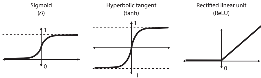
Figure 10.19 Three different activation functions used in neural networks. Left: The sigmoid function, represented by the Greek letter sigma . Middle: The hyperbolic tangent, or tanh. Right: The rectified linear unit, or ReLU.
