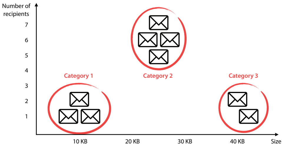
Figure 2.6 We can cluster the emails into three categories based on size and number of recipients.
