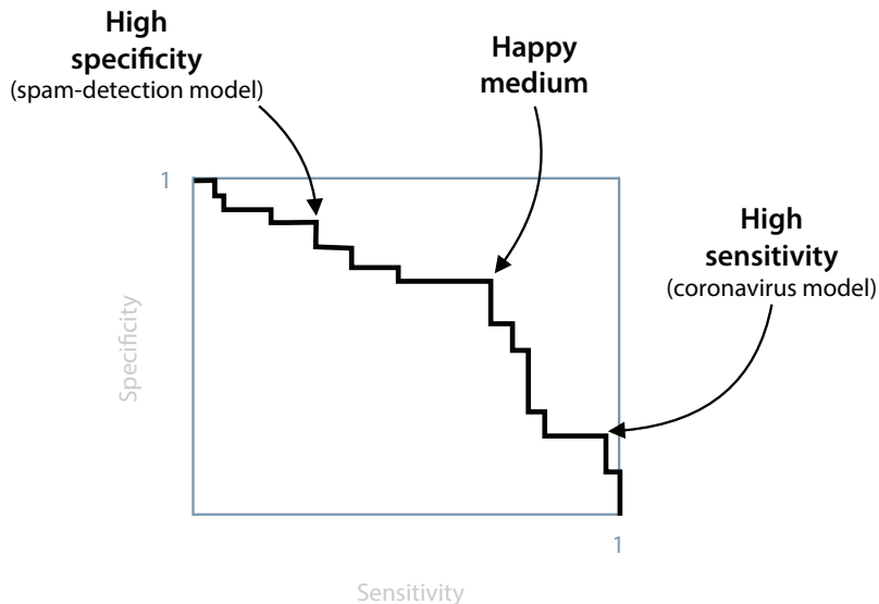
Figure 7.8 In this more general scenario, we can see an ROC curve and three points on it corresponding to three different thresholds. If we want to pick a threshold that gives us high specificity, we pick the one on the left. For a model with high sensitivity, we pick the one on the right. If we want a model that has a good amount of both sensitivity and specificity, we pick the one in the middle.
