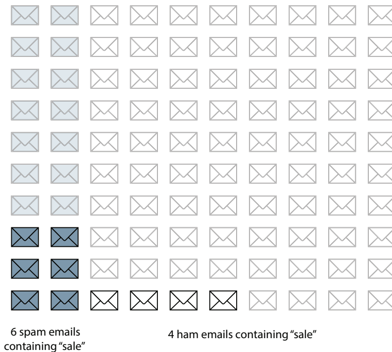
Figure 8.10 In a similar calculation as for the word lottery , we look at the emails containing the word sale . Among these (not grayed-out) emails, there are six spam and four ham.
